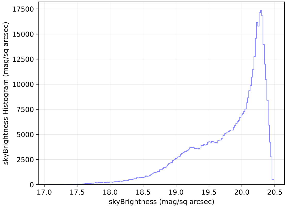
weather_cloudso12v3.4_10yrs WFD i band: skyBrightness Histogram
