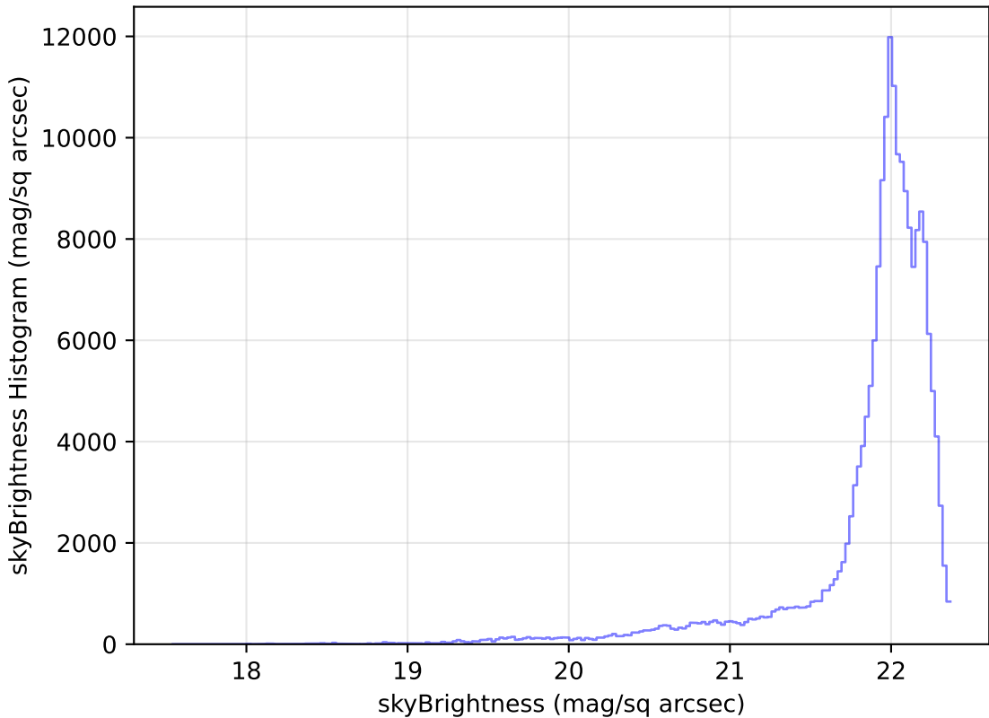
weather_cloudso12v3.4_10yrs WFD g band: skyBrightness Histogram
