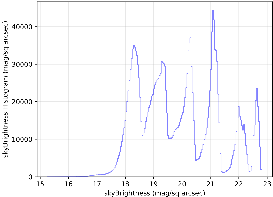
weather_cloudso12v3.4_10yrs WFD all bands: skyBrightness Histogram
