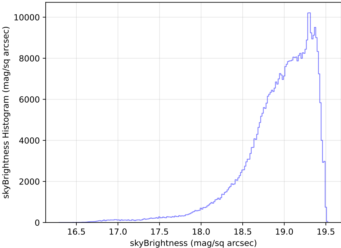
weather_cloudso12v3.4_10yrs All sky z band: skyBrightness Histogram
