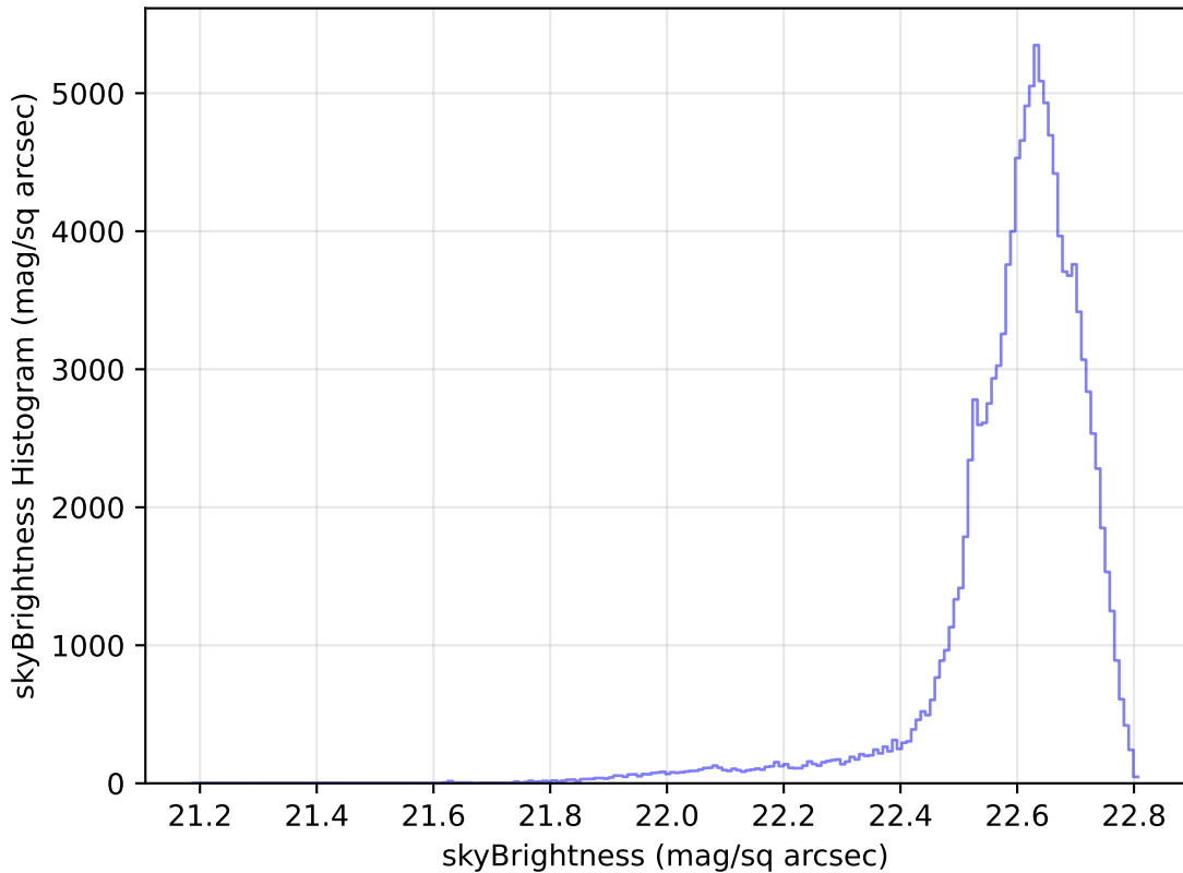
weather_cloudso12v3.4_10yrs All sky u band: skyBrightness Histogram
