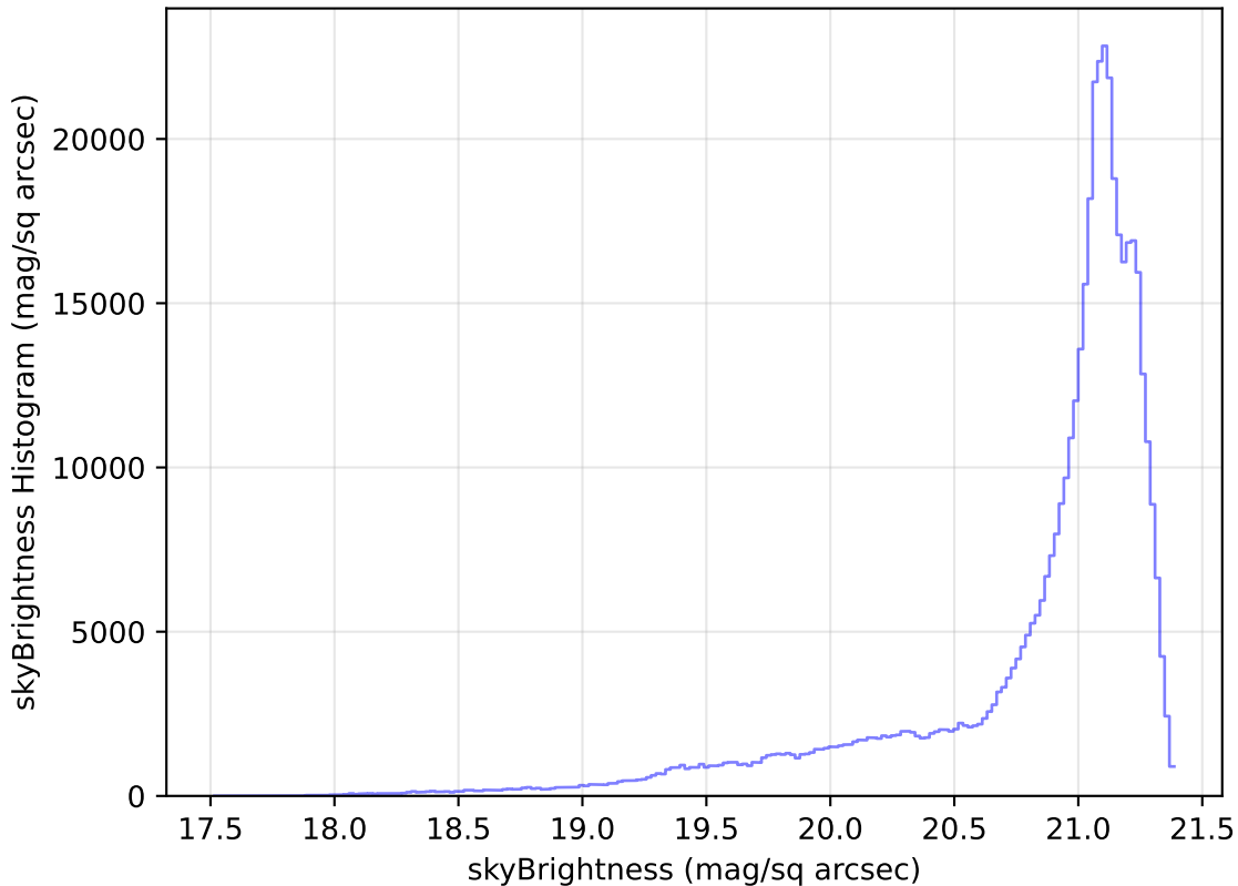
weather_cloudso12v3.4_10yrs All sky r band: skyBrightness Histogram
