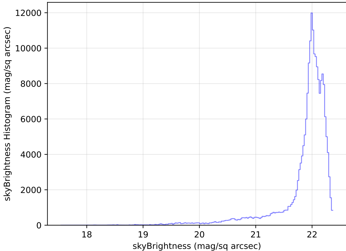
weather_cloudso12v3.4_10yrs All sky g band: skyBrightness Histogram
