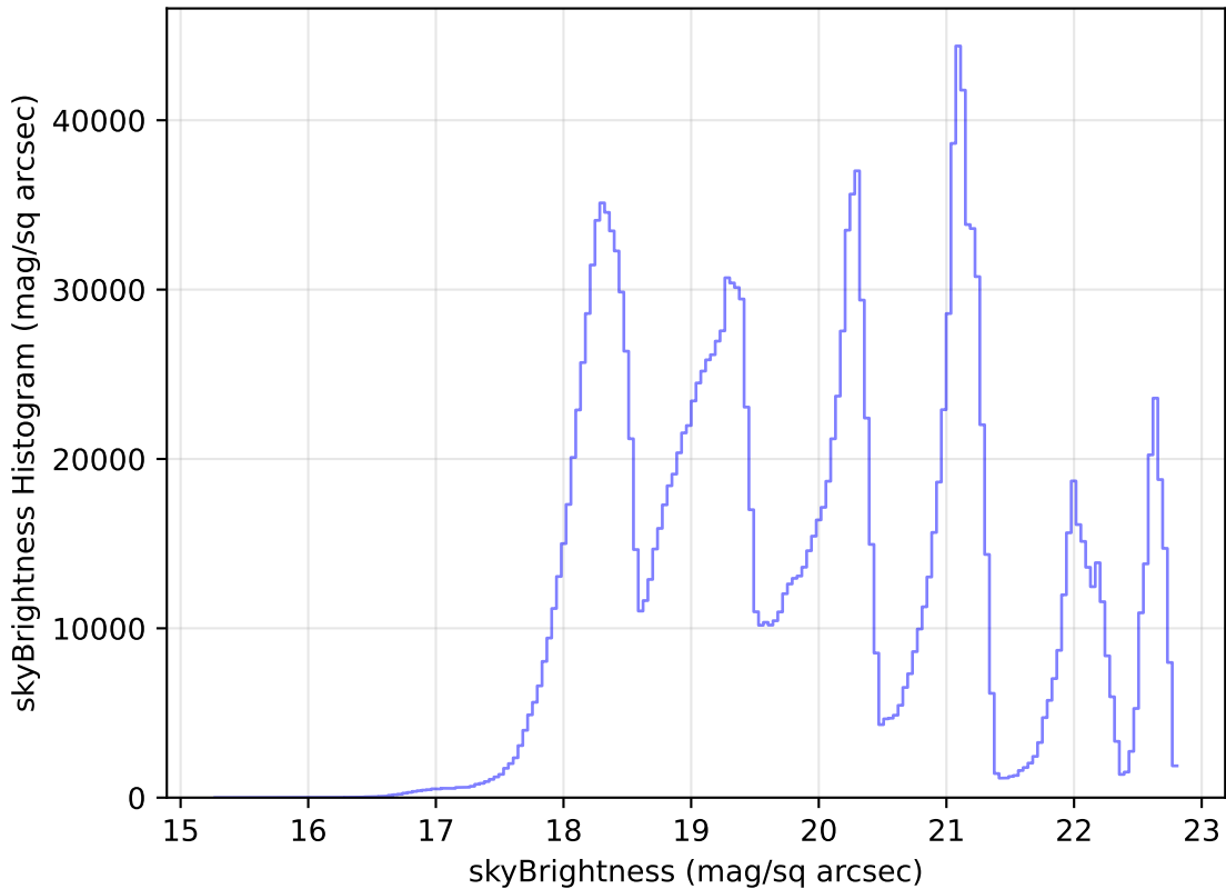
weather_cloudso12v3.4_10yrs All sky all bands: skyBrightness Histogram
