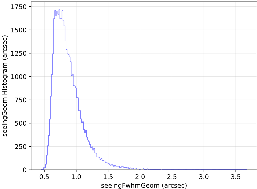
weather_cloudso12v3.4_10yrs Yr 1 z band: seeingGeom Histogram
