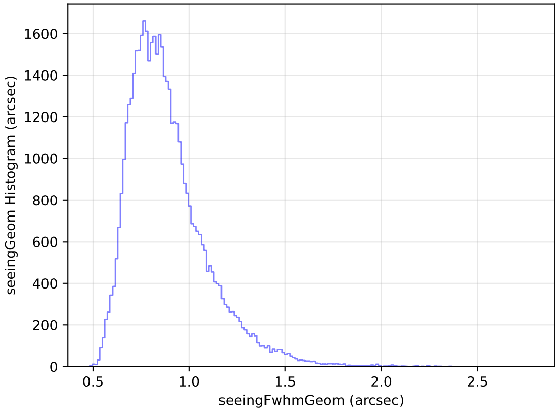
weather_cloudso12v3.4_10yrs Yr 1 y band: seeingGeom Histogram
