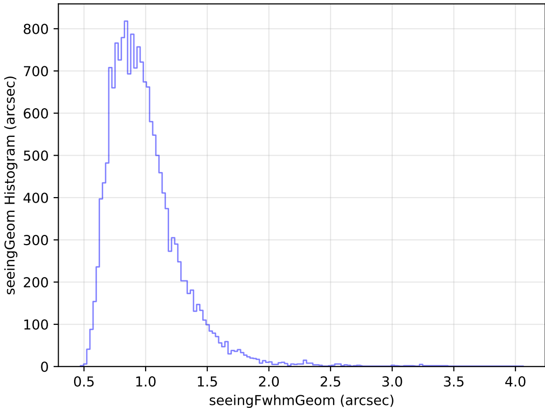
weather_cloudso12v3.4_10yrs Yr 1 u band: seeingGeom Histogram
