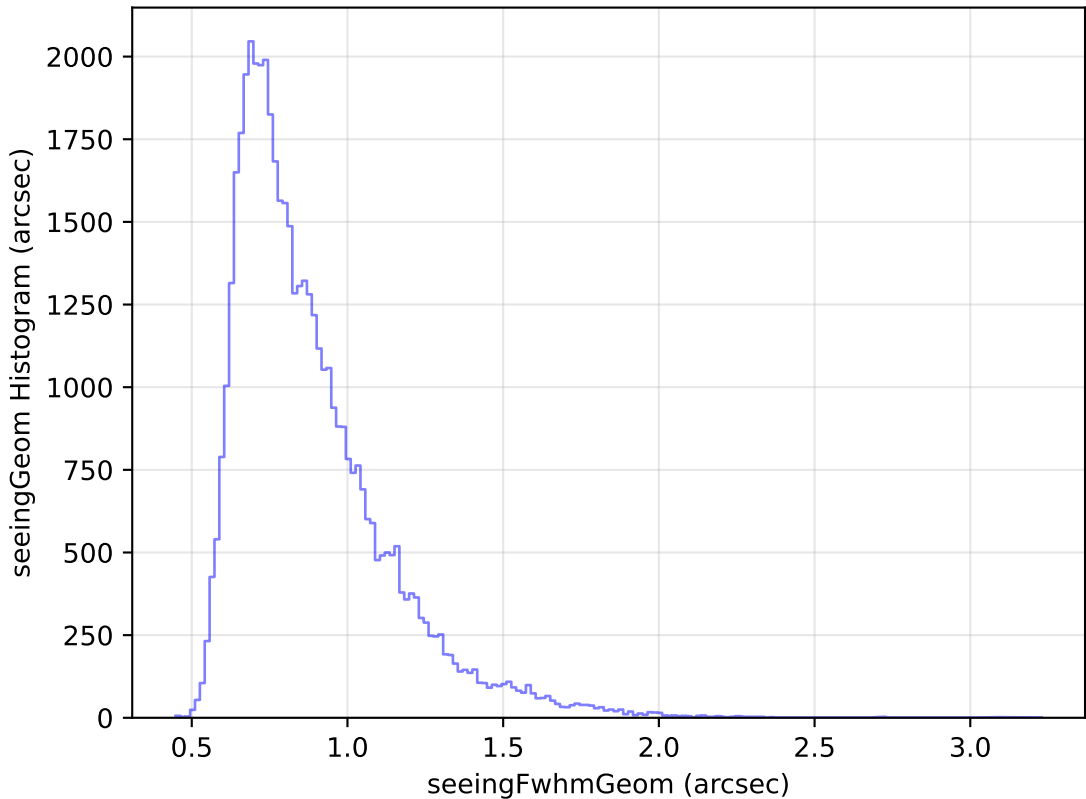
weather_cloudso12v3.4_10yrs Yr 1 r band: seeingGeom Histogram
