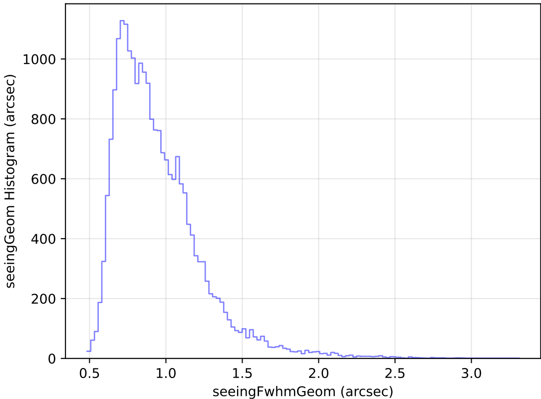
weather_cloudso12v3.4_10yrs Yr 1 g band: seeingGeom Histogram
