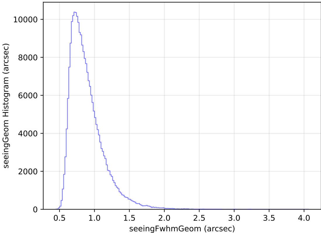
weather_cloudso12v3.4_10yrs Yr 1 all bands: seeingGeom Histogram
