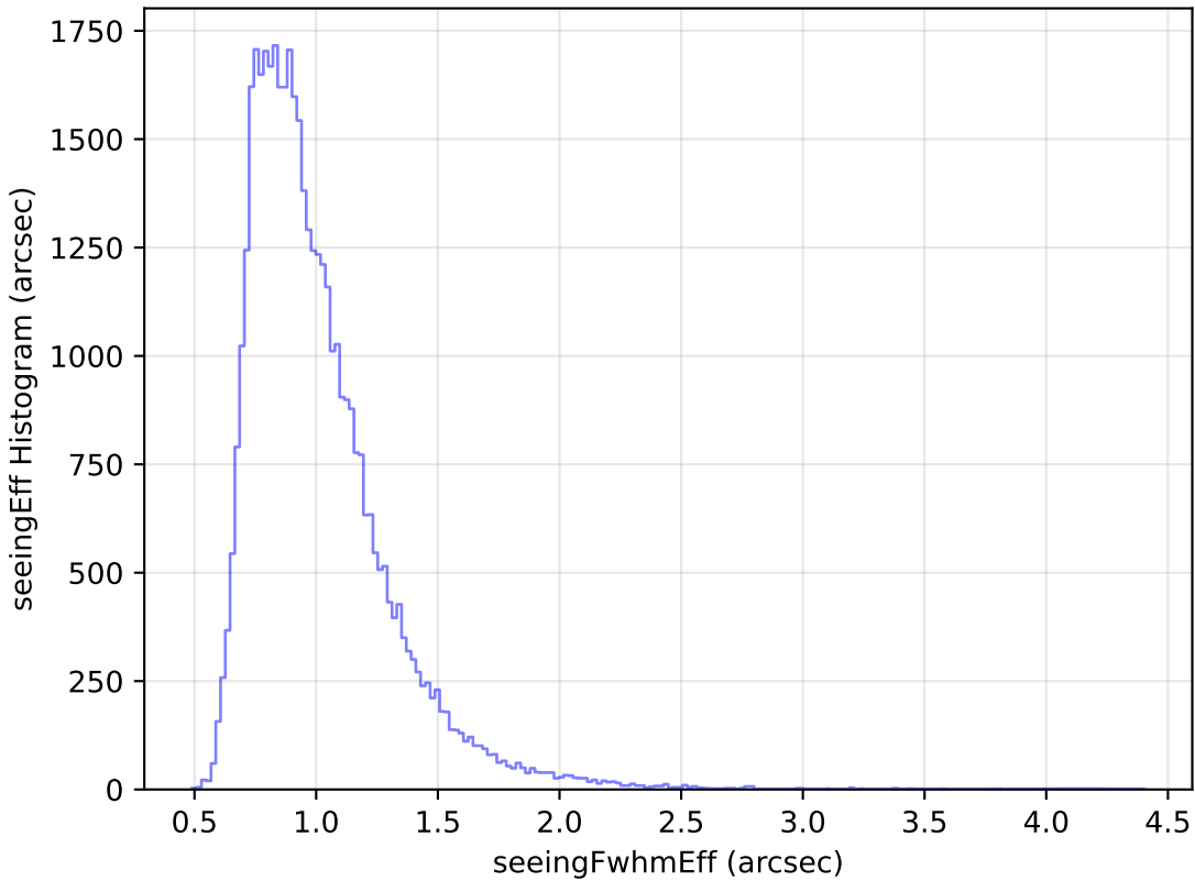
weather_cloudso12v3.4_10yrs Yr 1 z band: seeingEff Histogram
