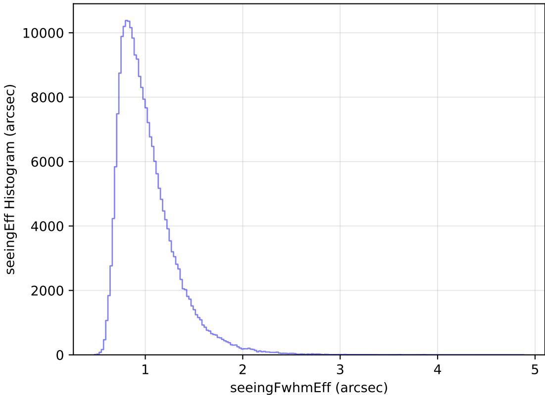
weather_cloudso12v3.4_10yrs Yr 1 all bands: seeingEff Histogram
