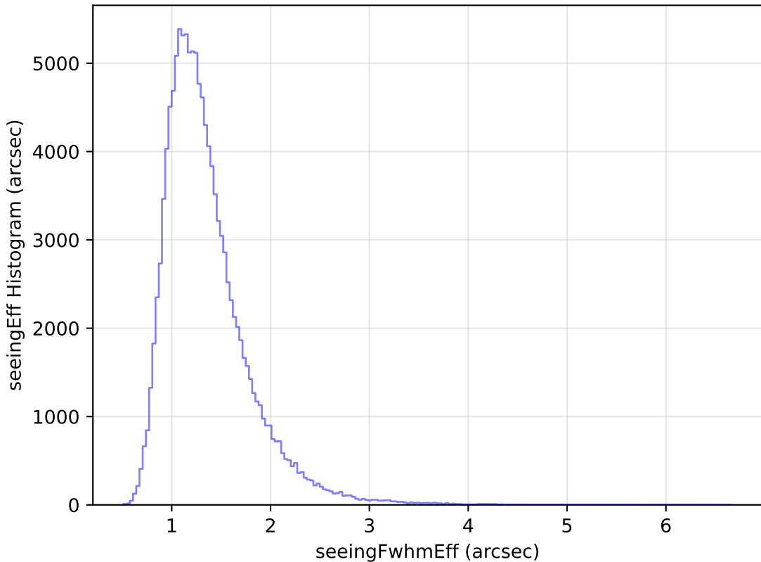
weather_cloudso12v3.4_10yrs WFD u band: seeingEff Histogram
