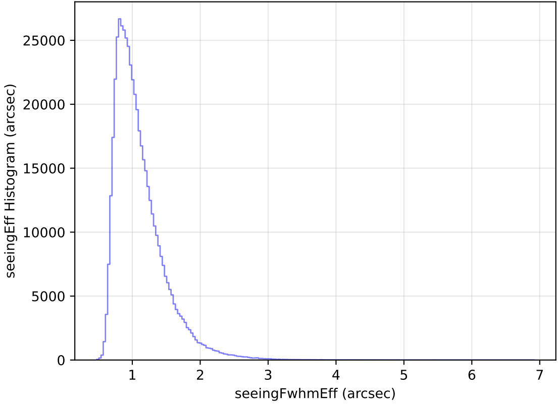
weather_cloudso12v3.4_10yrs WFD i band: seeingEff Histogram
