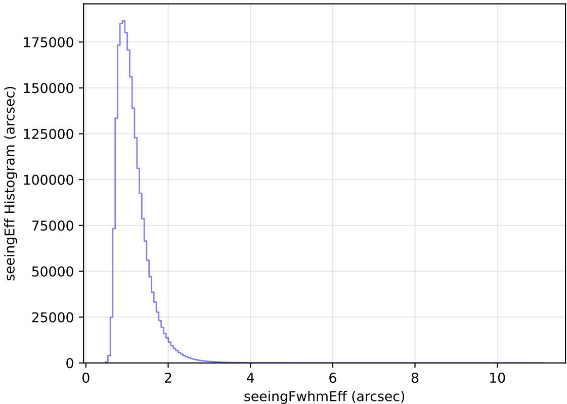
weather_cloudso12v3.4_10yrs WFD all bands: seeingEff Histogram
