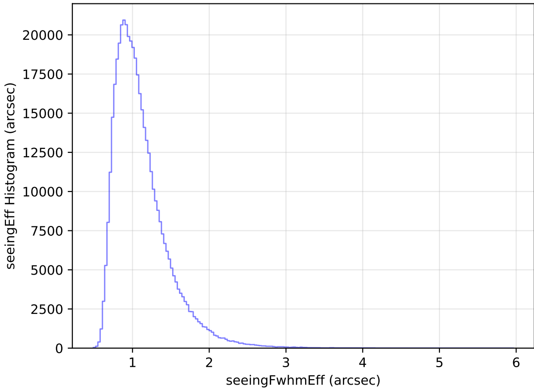
weather_cloudso12v3.4_10yrs All sky z band: seeingEff Histogram
