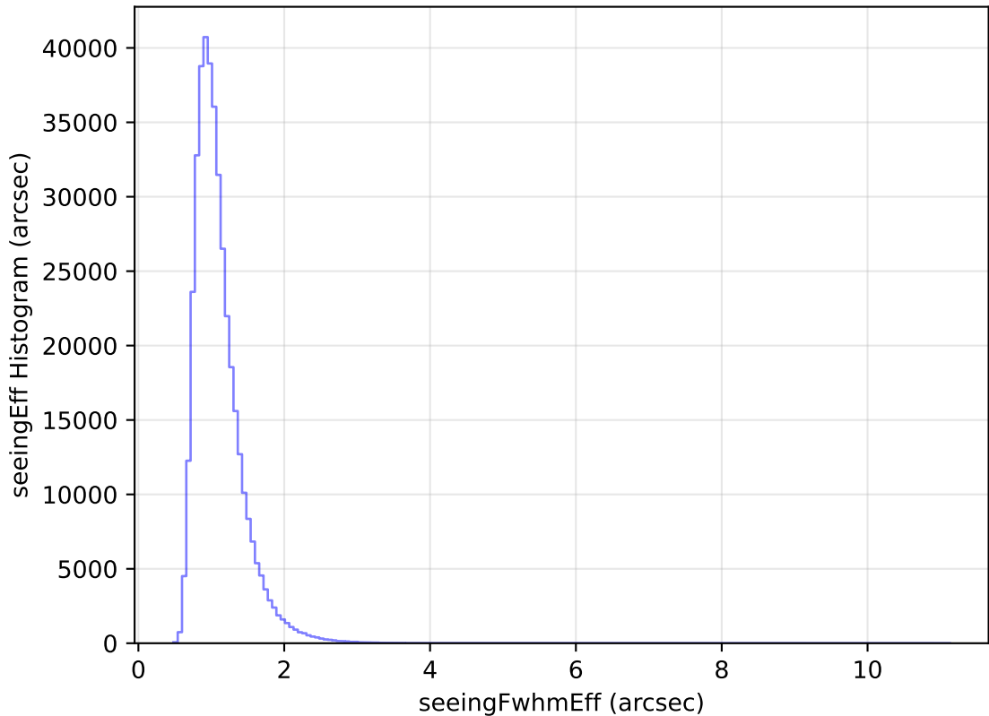
weather_cloudso12v3.4_10yrs All sky y band: seeingEff Histogram
