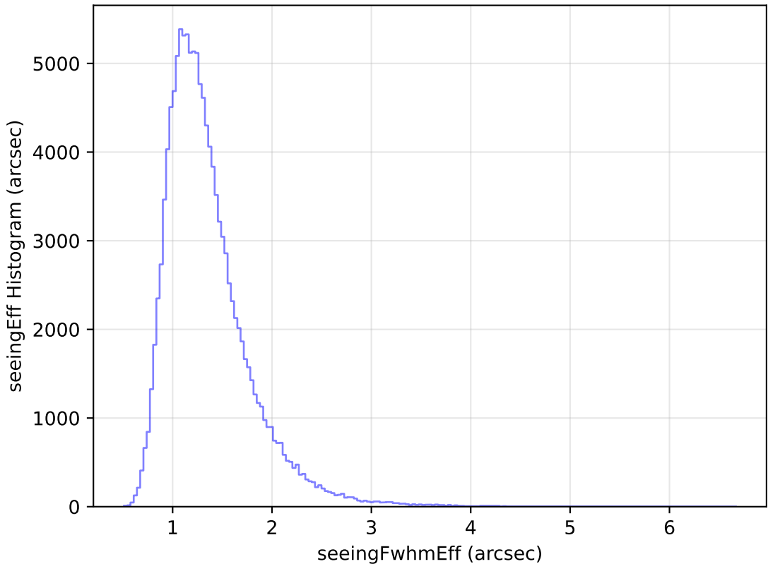
weather_cloudso12v3.4_10yrs All sky u band: seeingEff Histogram
