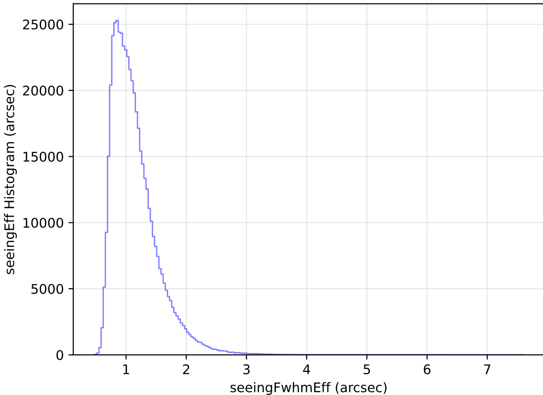
weather_cloudso12v3.4_10yrs All sky r band: seeingEff Histogram
