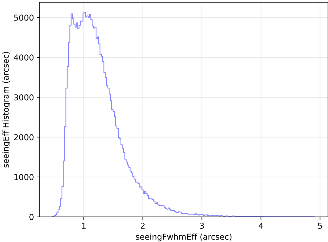
weather_cloudso12v3.4_10yrs All sky g band: seeingEff Histogram
