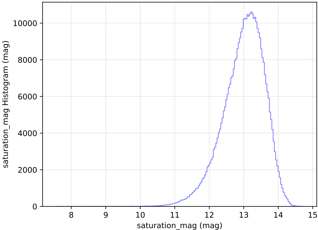
weather_cloudso12v3.4_10yrs WFD y band: saturation_mag Histogram
