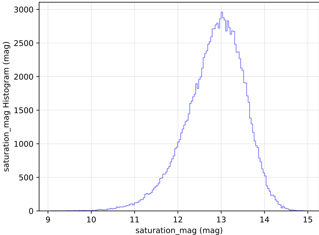
weather_cloudso12v3.4_10yrs WFD u band: saturation_mag Histogram
