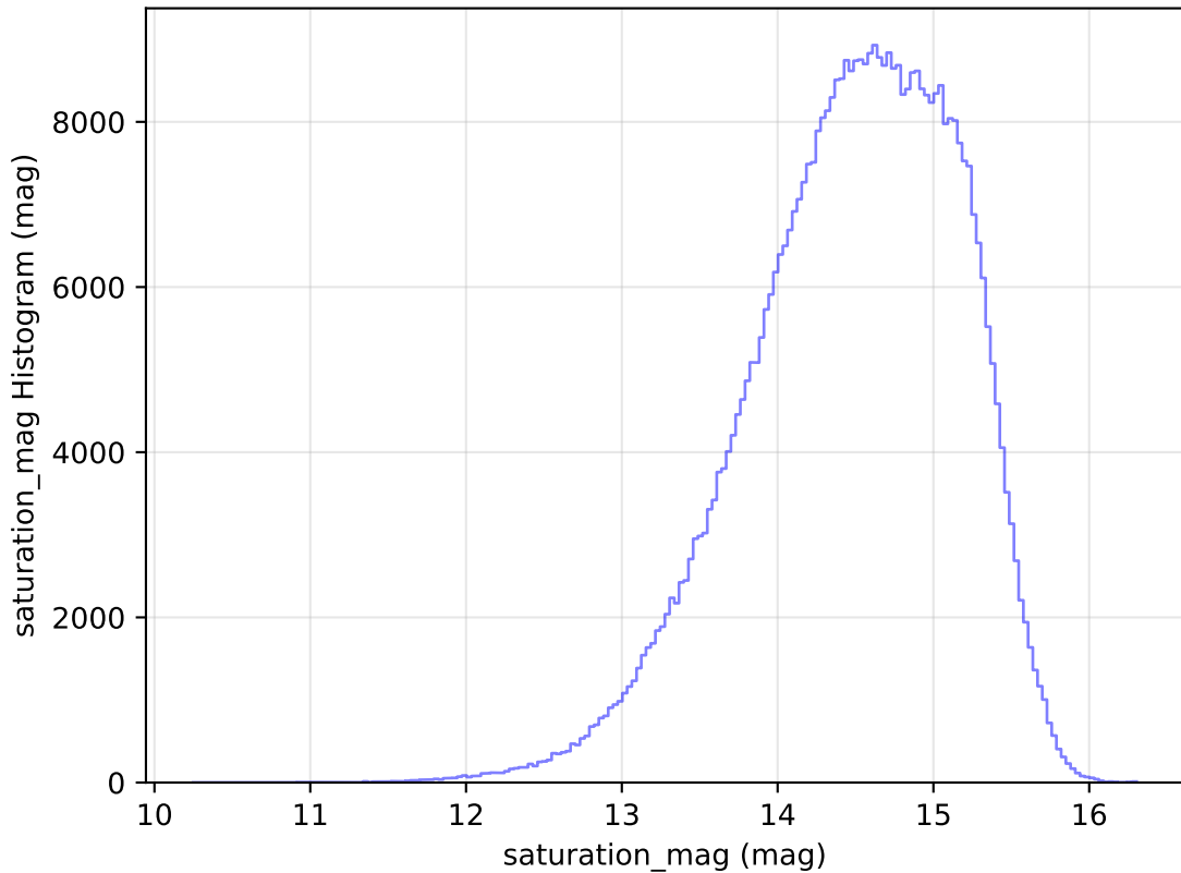
weather_cloudso12v3.4_10yrs WFD r band: saturation_mag Histogram
