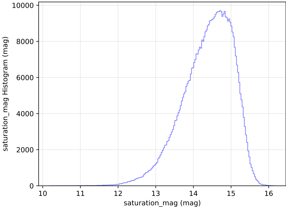
weather_cloudso12v3.4_10yrs WFD i band: saturation_mag Histogram
