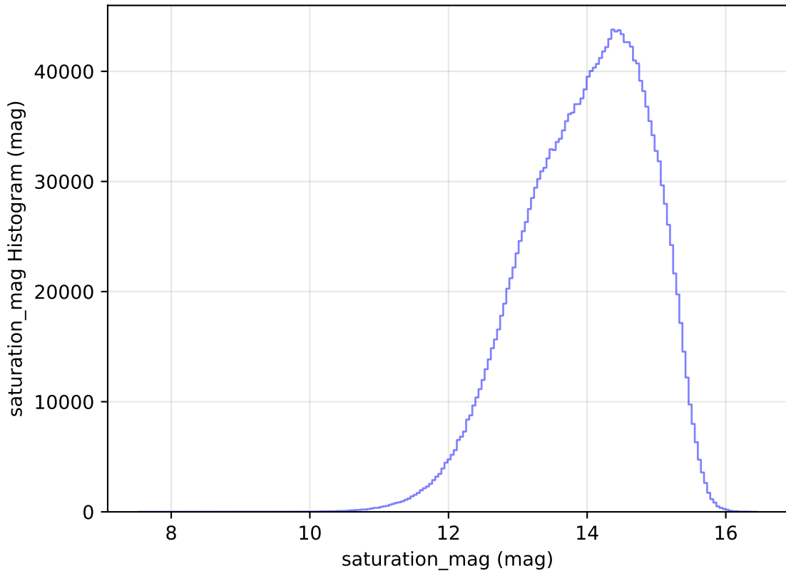
weather_cloudso12v3.4_10yrs WFD all bands: saturation_mag Histogram
