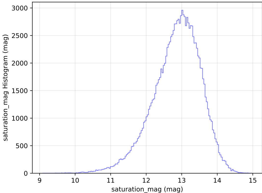
weather_cloudso12v3.4_10yrs All sky u band: saturation_mag Histogram
