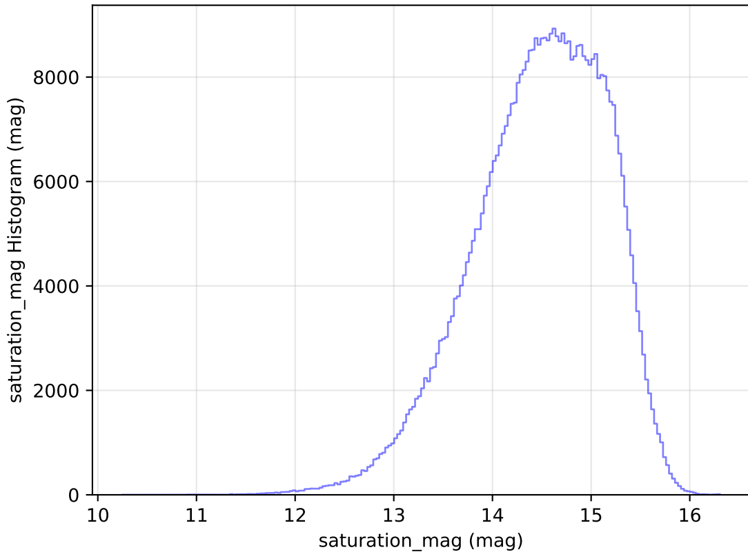
weather_cloudso12v3.4_10yrs All sky r band: saturation_mag Histogram
