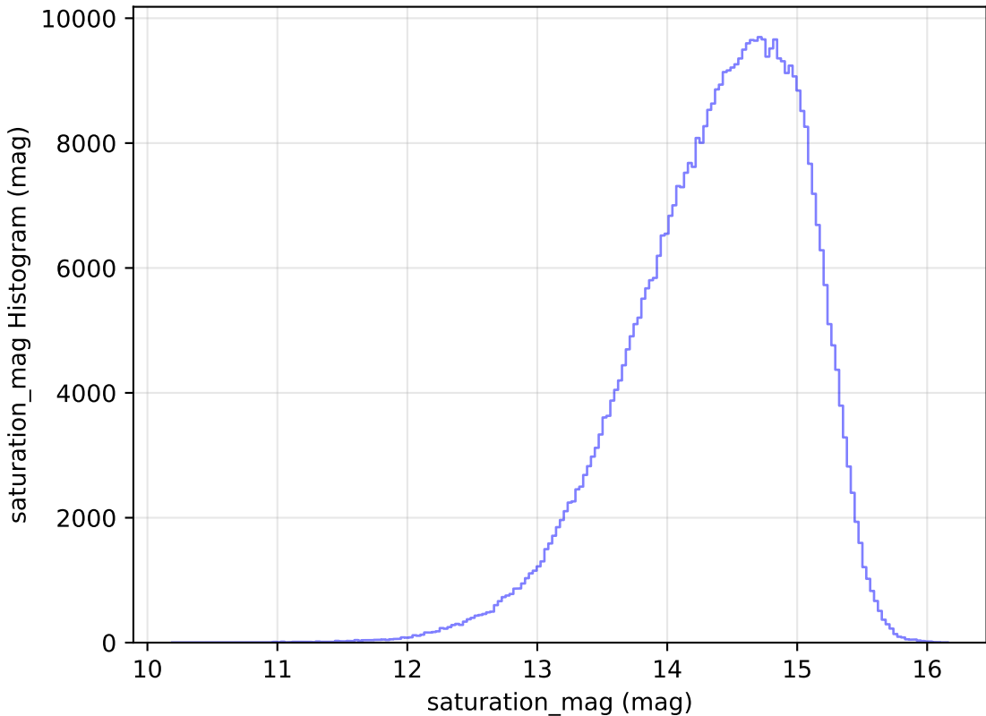
weather_cloudso12v3.4_10yrs All sky i band: saturation_mag Histogram
