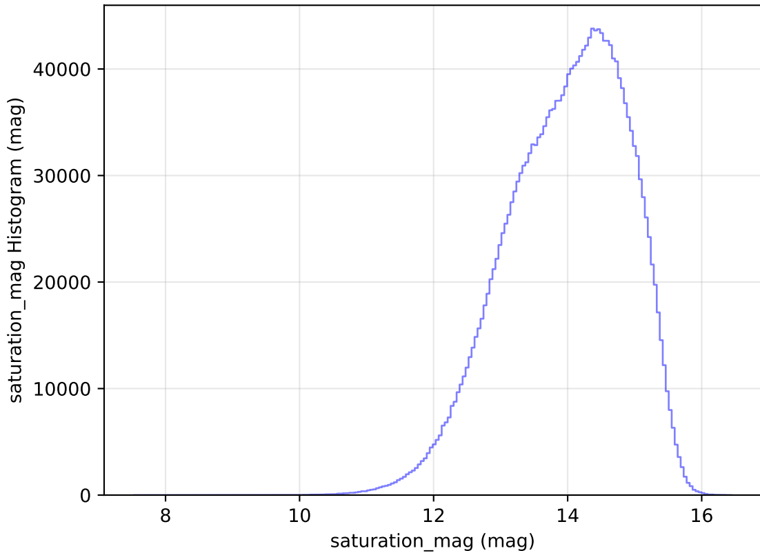
weather_cloudso12v3.4_10yrs All sky all bands: saturation_mag Histogram
