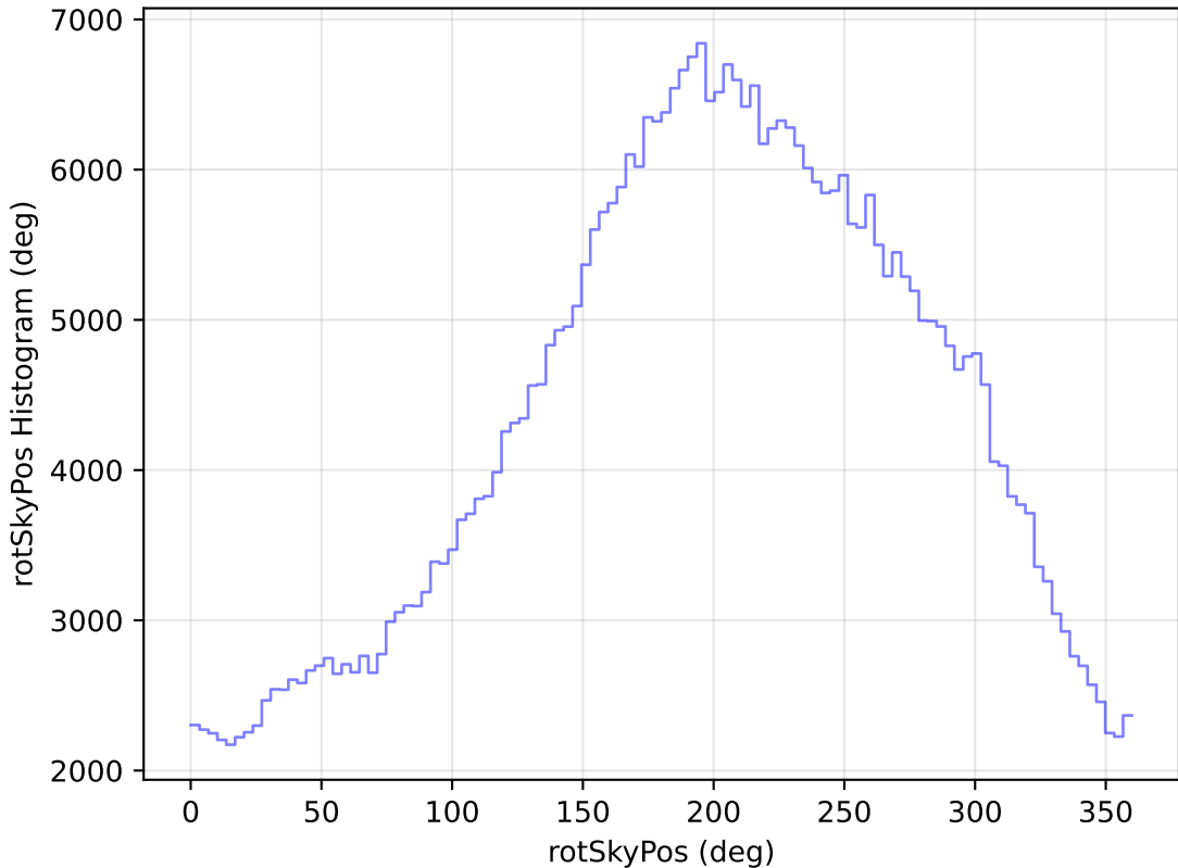
weather_cloudso12v3.4_10yrs WFD z band: rotSkyPos Histogram
