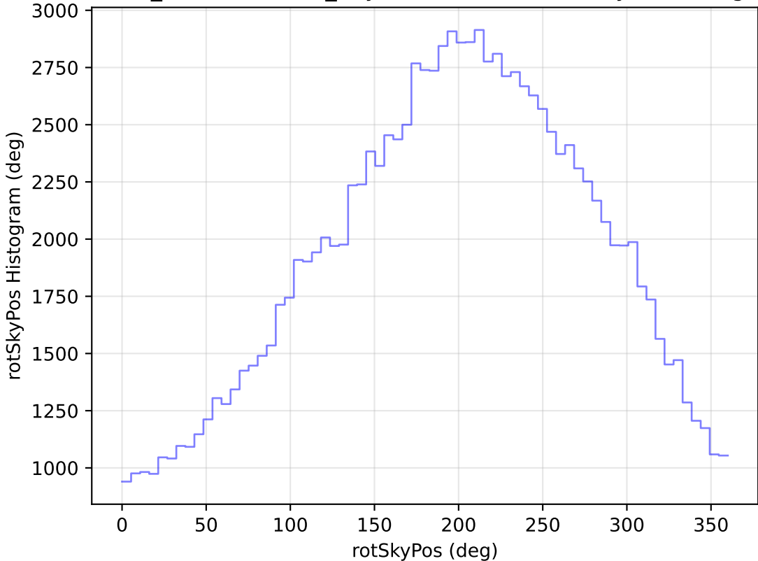
weather_cloudso12v3.4_10yrs WFD u band: rotSkyPos Histogram
