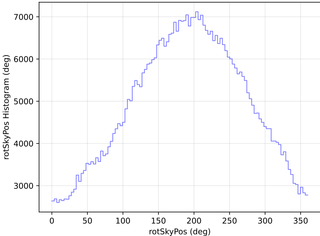
weather_cloudso12v3.4_10yrs WFD r band: rotSkyPos Histogram
