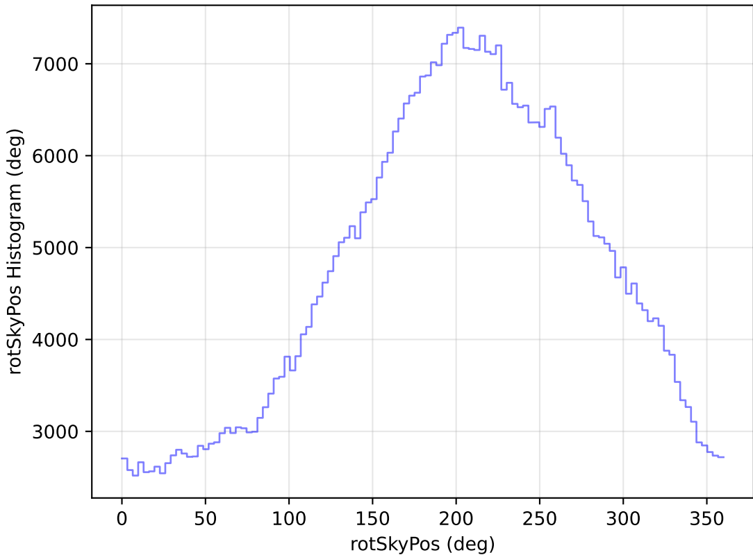
weather_cloudso12v3.4_10yrs WFD i band: rotSkyPos Histogram
