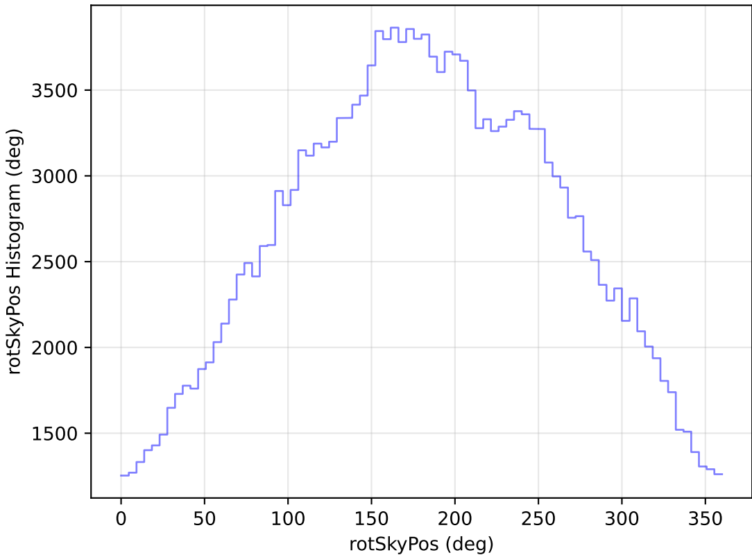
weather_cloudso12v3.4_10yrs WFD g band: rotSkyPos Histogram
