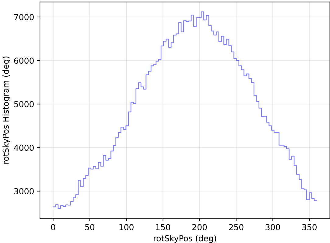
weather_cloudso12v3.4_10yrs All sky r band: rotSkyPos Histogram
