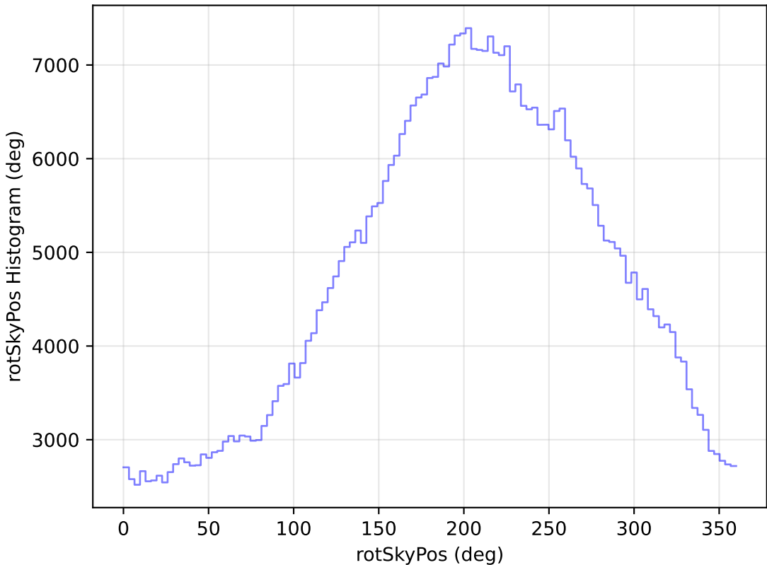
weather_cloudso12v3.4_10yrs All sky i band: rotSkyPos Histogram
