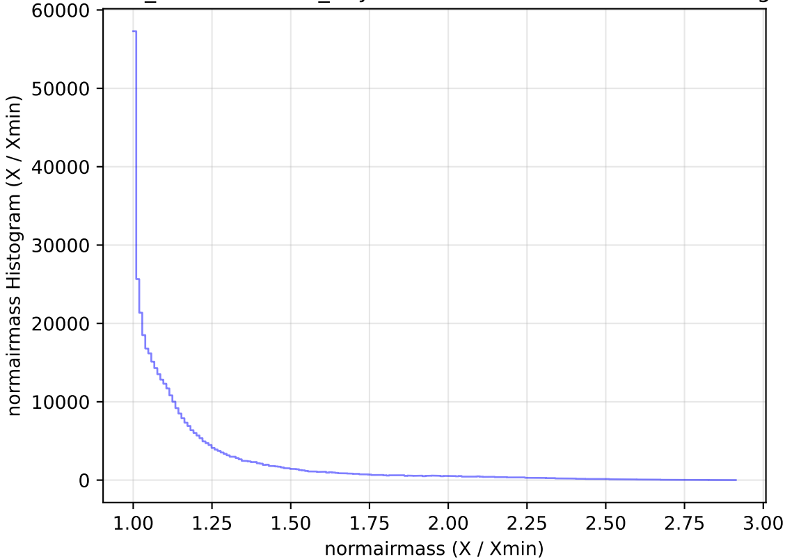
weather_cloudso12v3.4_10yrs WFD z band: normairmass Histogram
