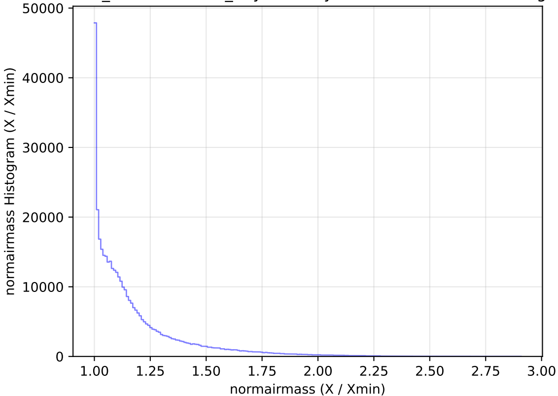
weather_cloudso12v3.4_10yrs WFD y band: normairmass Histogram
