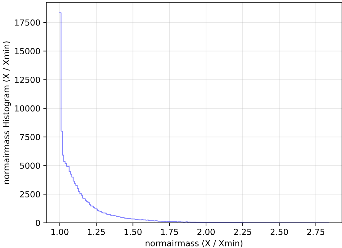
weather_cloudso12v3.4_10yrs WFD u band: normairmass Histogram
