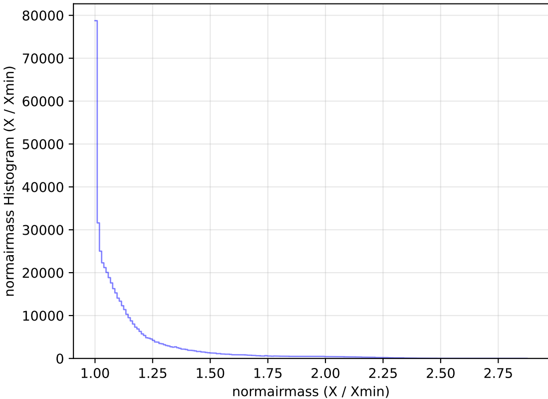
weather_cloudso12v3.4_10yrs WFD r band: normairmass Histogram
