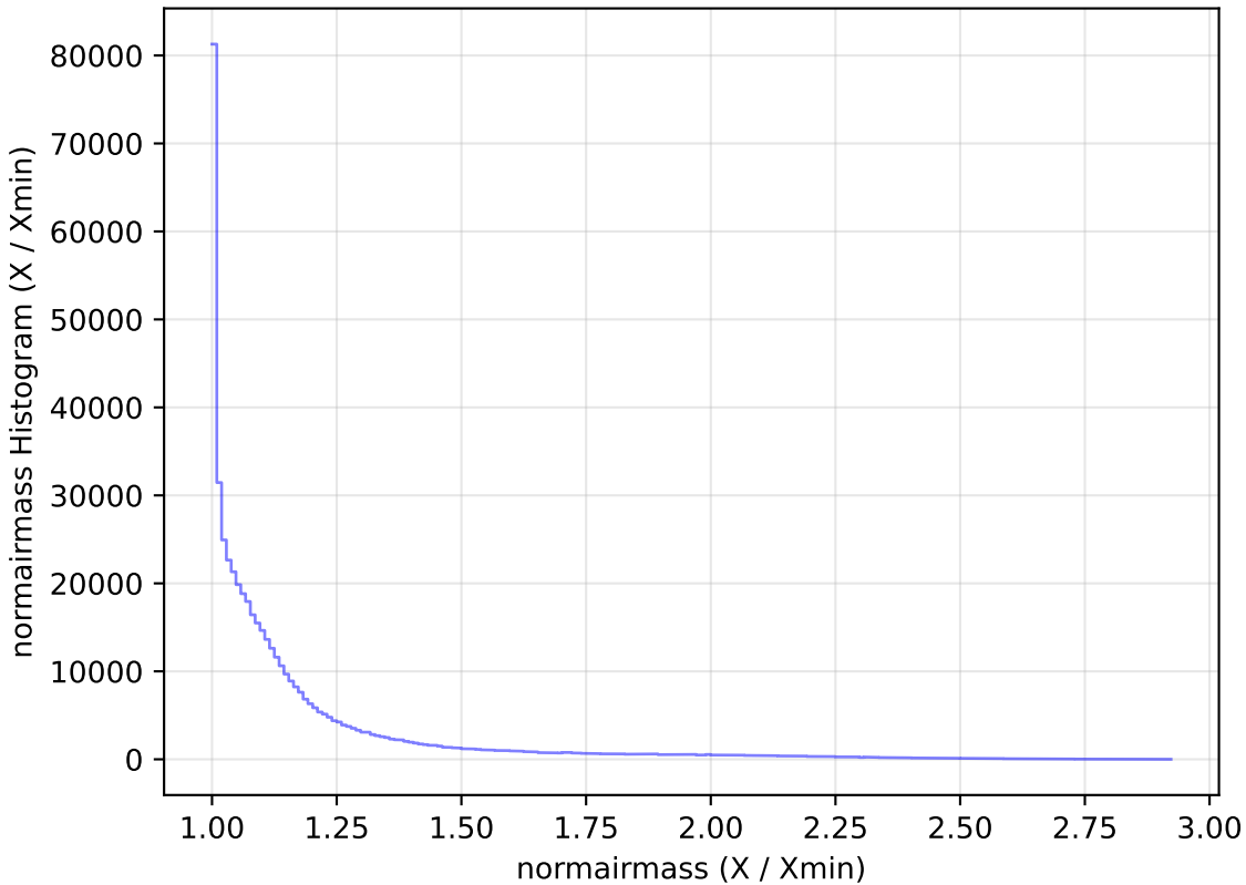
weather_cloudso12v3.4_10yrs WFD i band: normairmass Histogram
