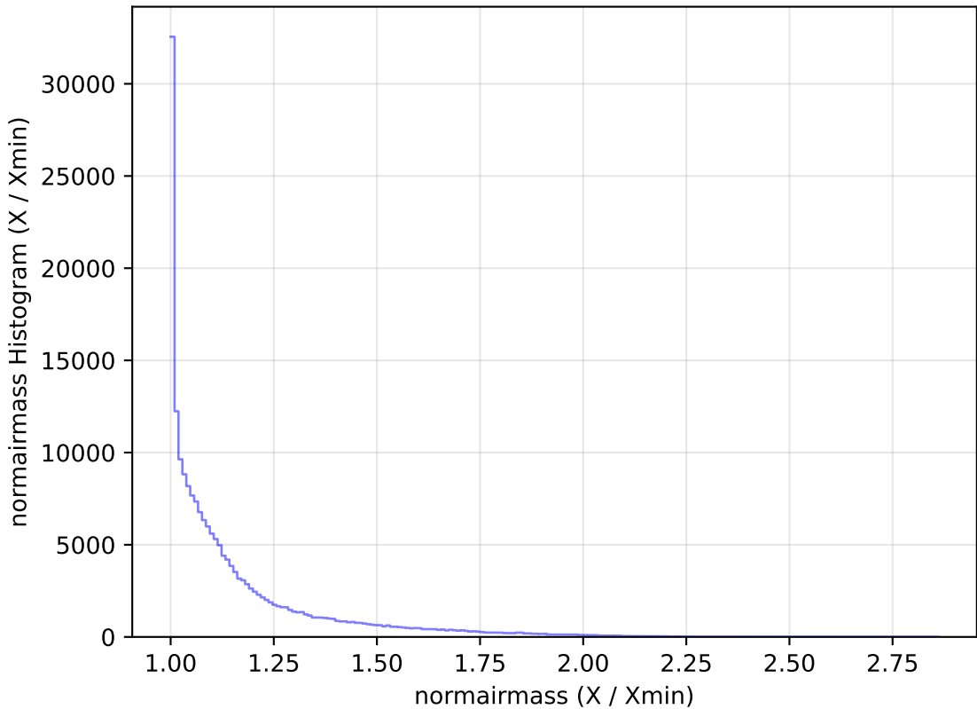
weather_cloudso12v3.4_10yrs WFD g band: normairmass Histogram
