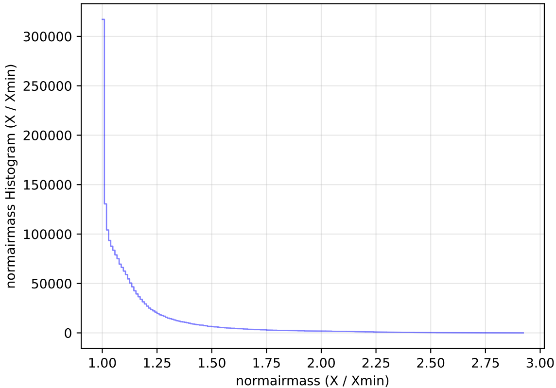
weather_cloudso12v3.4_10yrs WFD all bands: normairmass Histogram
