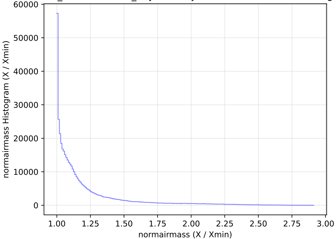
weather_cloudso12v3.4_10yrs All sky z band: normairmass Histogram
