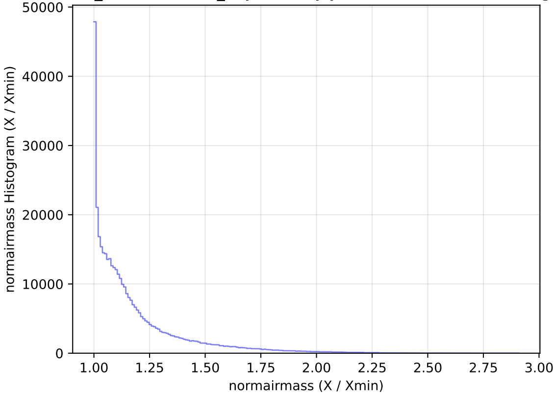
weather_cloudso12v3.4_10yrs All sky y band: normairmass Histogram
