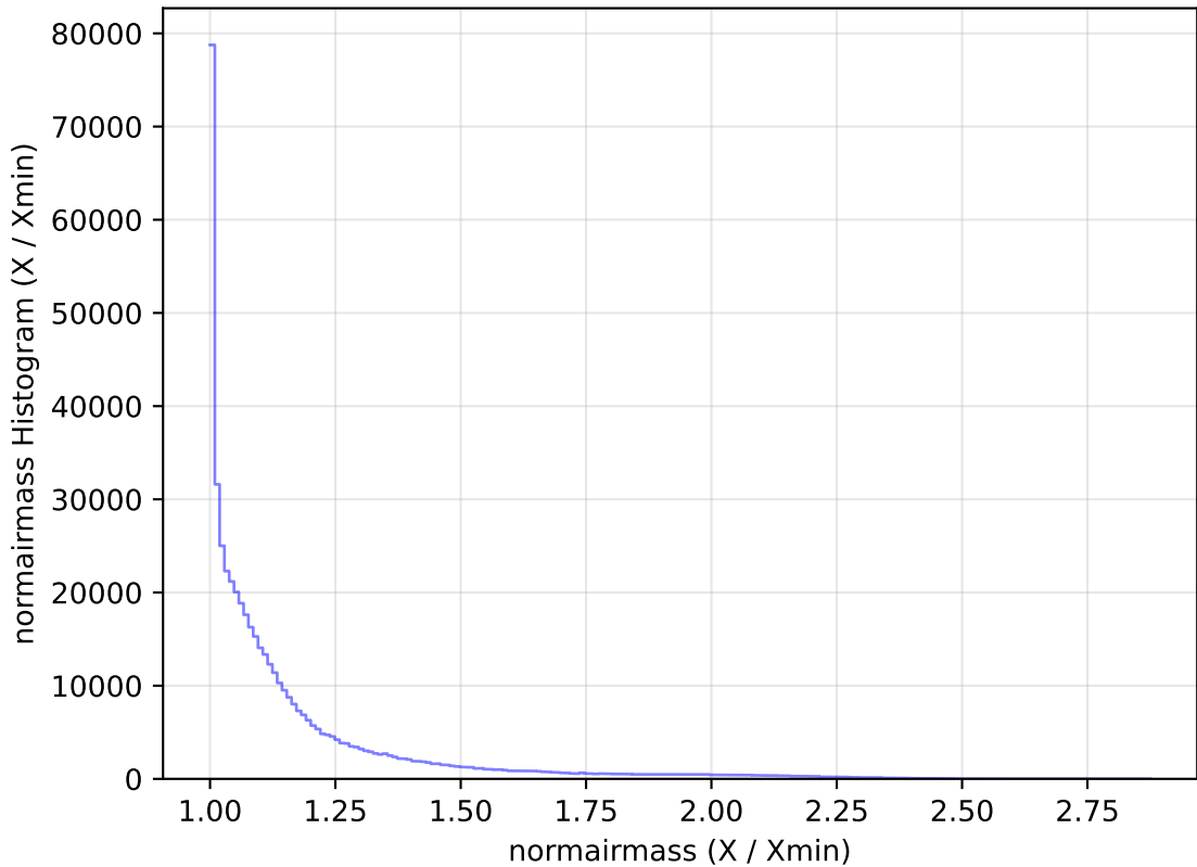
weather_cloudso12v3.4_10yrs All sky r band: normairmass Histogram
